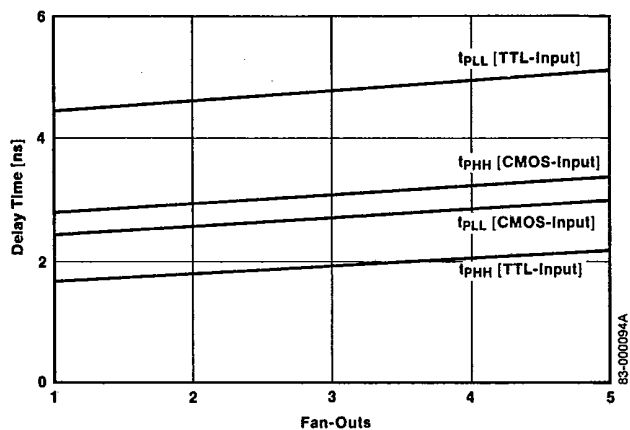
Delay Time vs Fan-Outs [Input Buffer]
