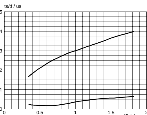
Fig. 10. Typical collector storage and fall time. t_s = f(I_B) ; t_f = f(I_B) ; I_C = 4.5 A; T_J = 85^\circ\text{C} ; f = 56 kHz
