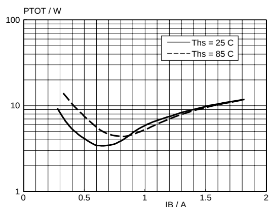
Fig. 9. Typical losses. P_{TOT} = f(I_B) ; I_C = 4.5 A; f = 56 kHz
