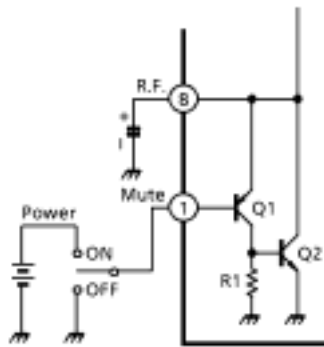
Fig.4 Mute circuit
