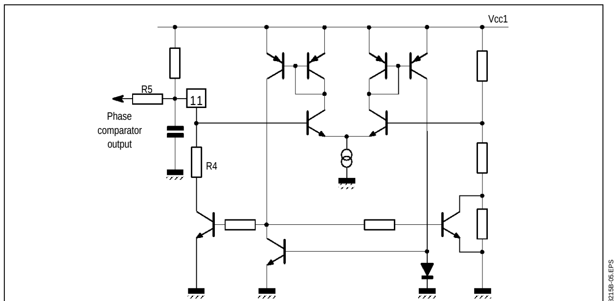
Figure 3 : Line Oscillator
