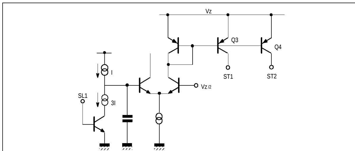
Figure 2 : Frame Separator
