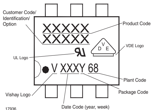
Figure 15. Marking example
