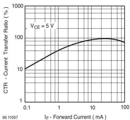
Figure 12. Current Transfer Ratio vs. Forward Current
