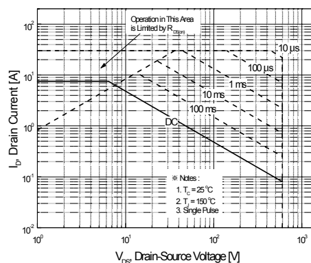
Figure 9-2. Maximum Safe Operating Area for FQPF8N60C
