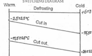
SWITCHING DIAGRAM
