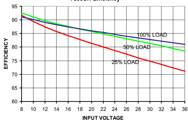
7805SR Efficiency
