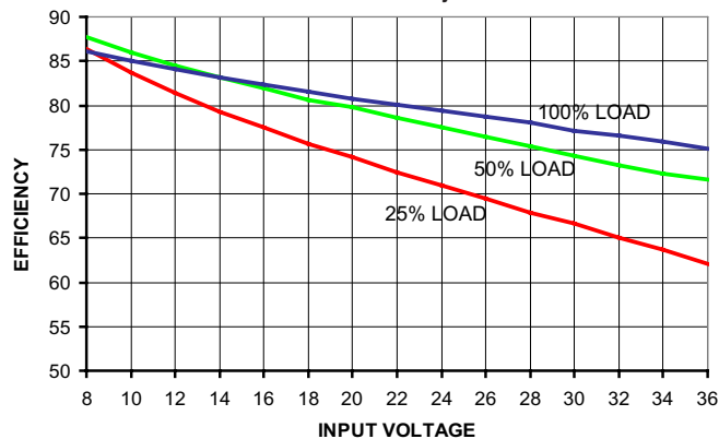
7803SR Efficiency
