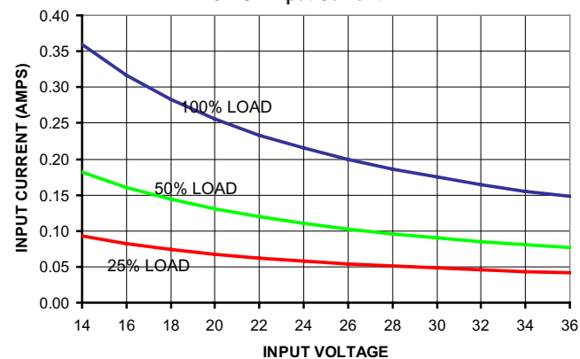
7812SR Input Current
