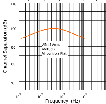
Fig.10 Input Separation (L1,L2,L3,L4) vs. Frequency
