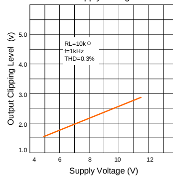
Fig.12 Output Clipping Level vs. Supply Voltage
