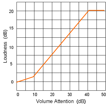
Fig.1 Loudness vs. Volume Attention
