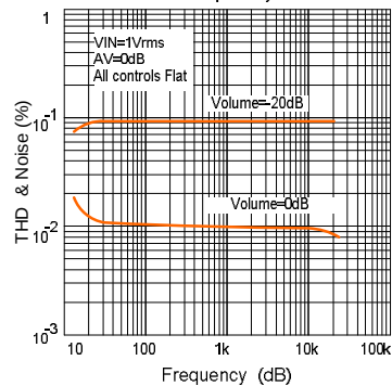
Fig.6 Distortion & Noise vs. Frequency
