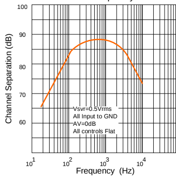
Fig.11 Supply Voltage Rejection vs. Frequency
