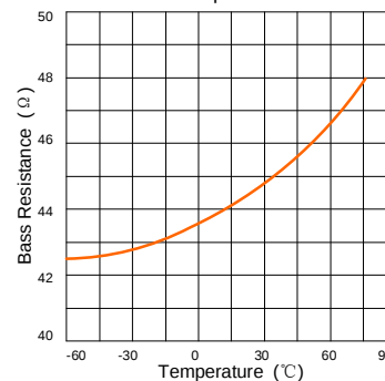
Fig.15 Bass resistance vs. Temperature
