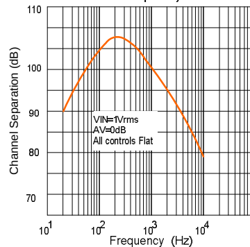
Fig.9 Channel Separation(L→R) vs. Frequency
