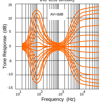
Fig.16 Typical Tone Response (with the Ext components indicated the test circuit)
